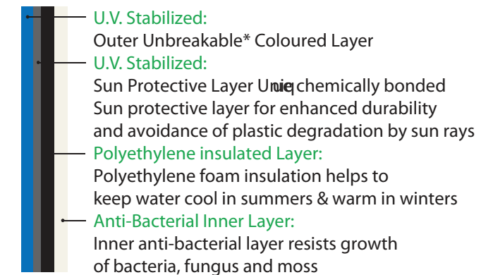
Cross Section of four layered Polyfoam Tank
